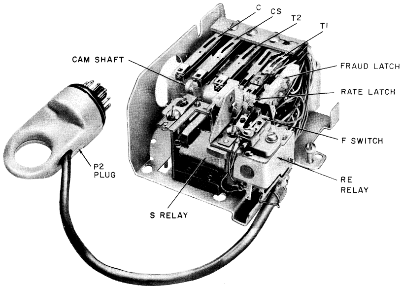
VIEW A
